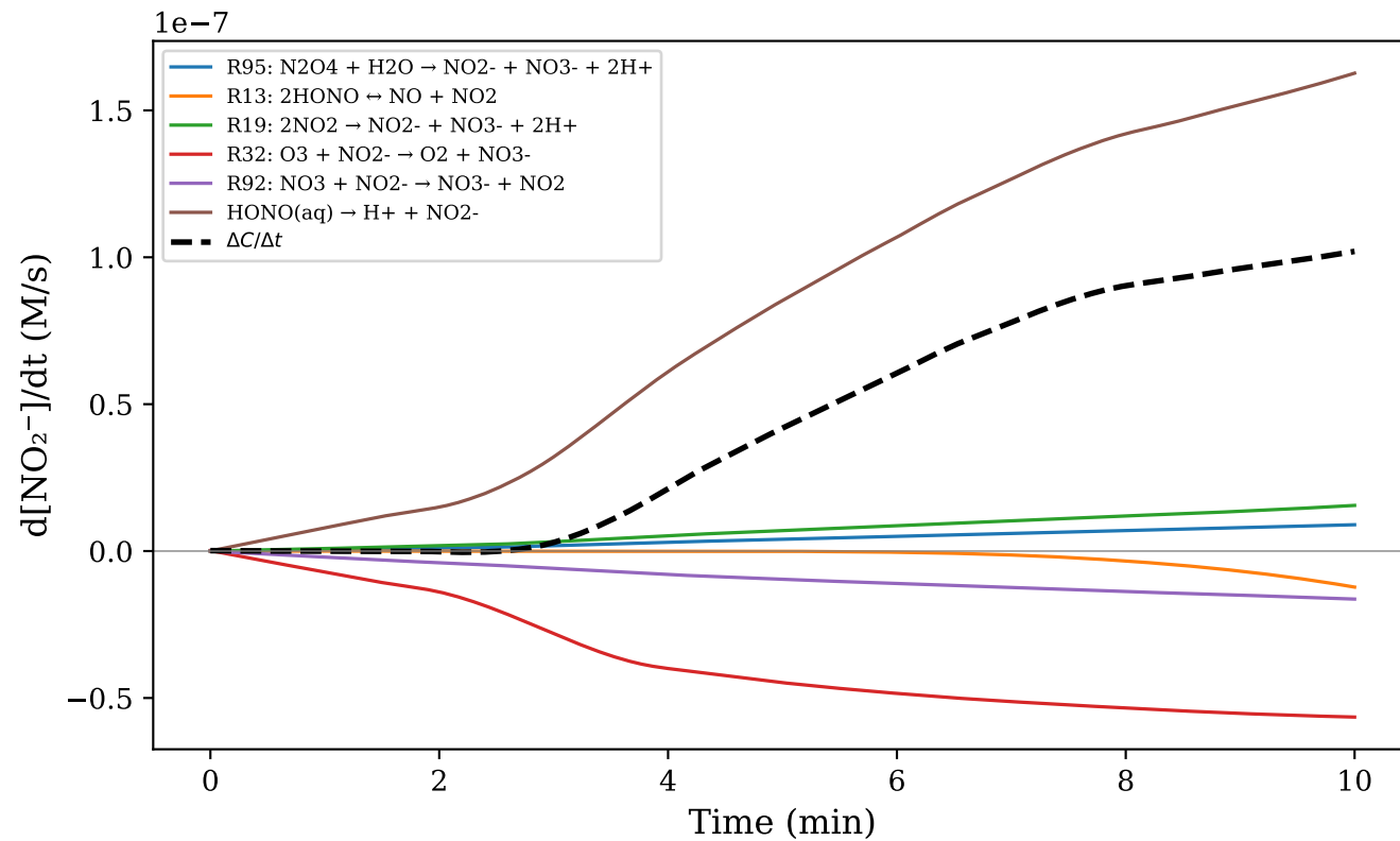
(c) \text{NO}_2^-
